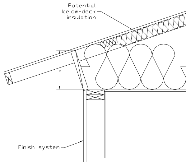
Figure 1010 9 : Section at Attic Edge with a Raised Heel Truss
