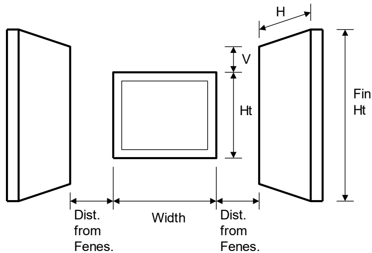
Figure 776: Sidefin Dimensions
