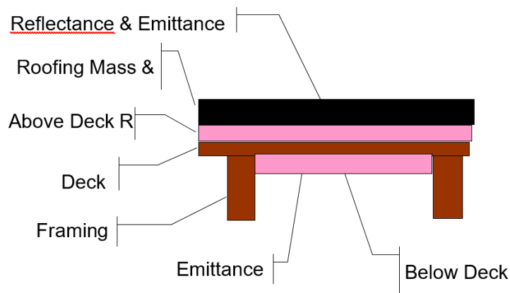
Figure 1111 10: Components of the Attic Through Roof Deck
