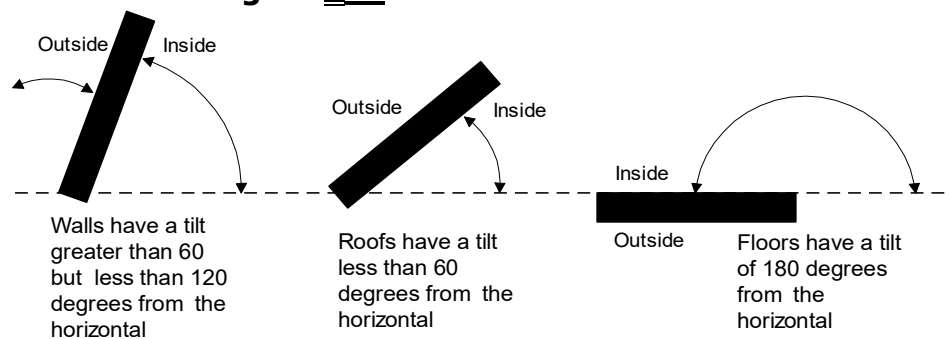
Figure 433 4: Surface Definitions
