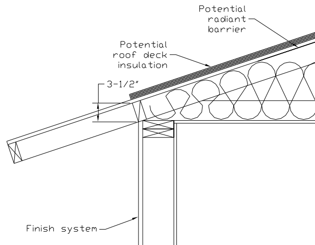
Figure 998: Section at Attic Edge with Standard Truss
