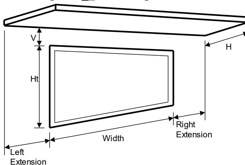
Figure 665: Overhang Dimensions
