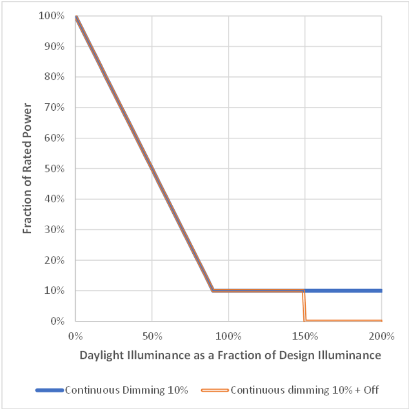
Figure 4777 8: Example of Lighting Power Fraction Continuous Dimming and Continuous Dimming Plus OFF Daylighting Controls (with Minimum Dimming Fraction of 10 Percent)
