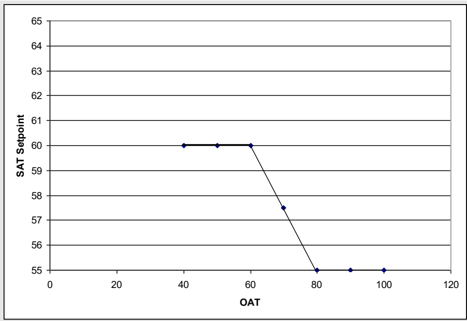
Figure 7.10.10.1.1: SAT Cooling Setpoint Reset Based on Outdoor Air Temperature (OAT)
