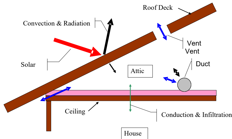
Figure 14 17 17 16 : Attic Model Components
