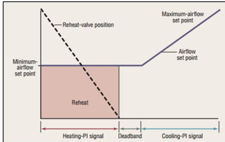
Figure 5889: Single Maximum VAV Box Control
