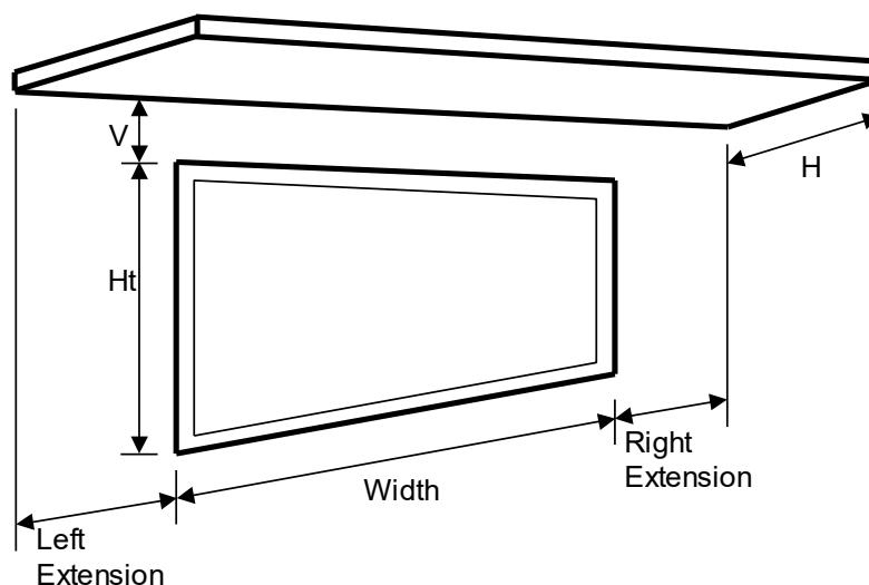
Figure 12151514 12151514: Overhang Dimensions
