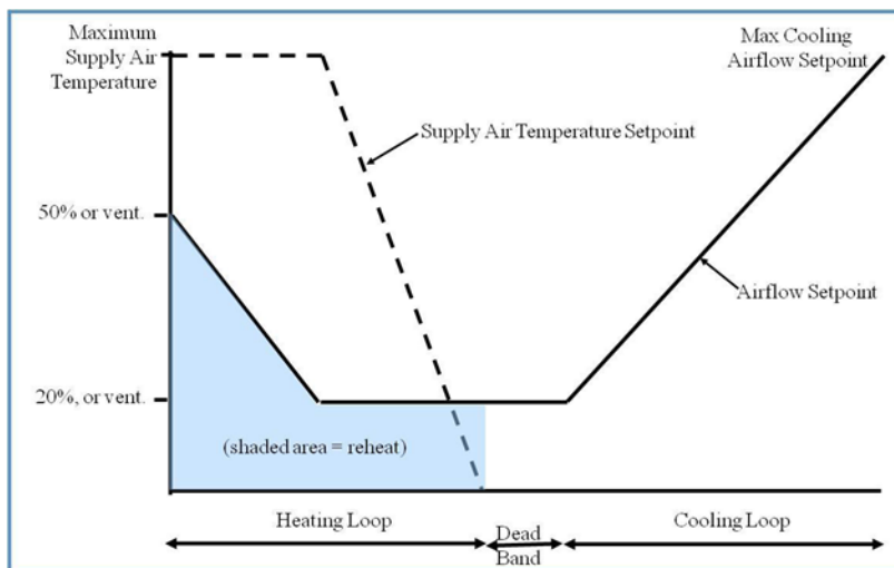
Figure 6-9.10: Dual Maximum Control Sequence
