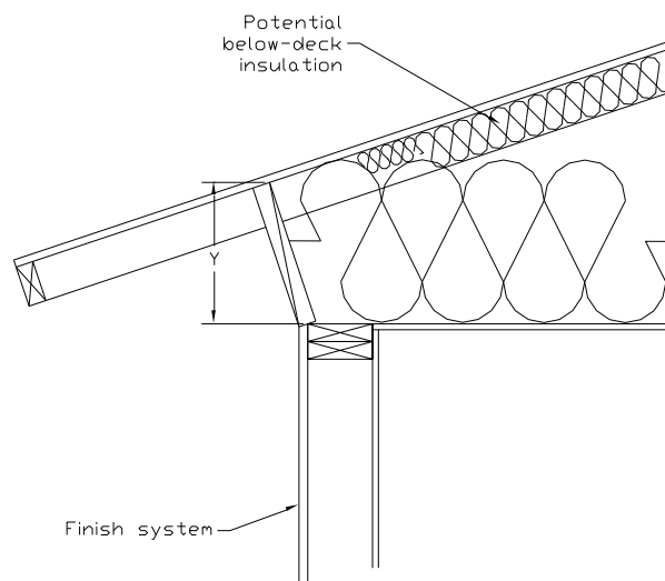
Figure 1619191918 : Section at Attic Edge with a Raised Heel Truss
