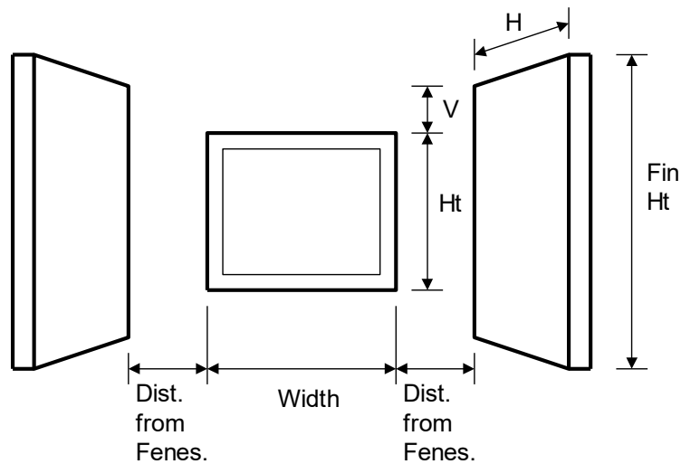
Figure 13.16.16.15: Sidesfin Dimensions
