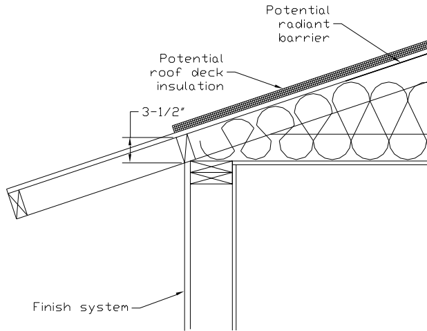
Figure 1518181817 : Section at Attic Edge with Standard Truss
